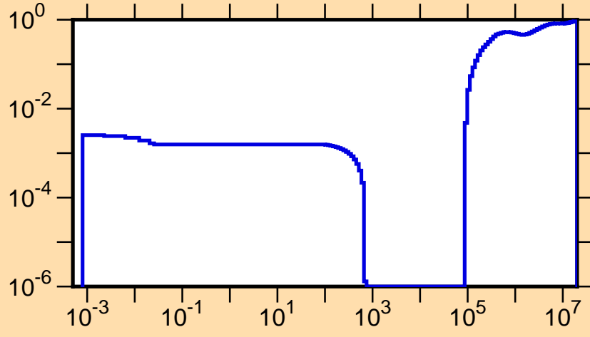
\mu vs. E for ^{258}
