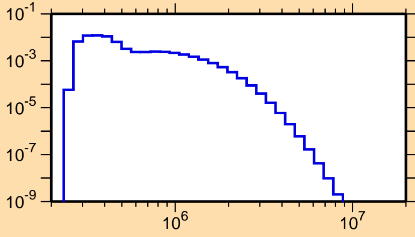
\sigma vs. E for ^{258}\text{Pu}
