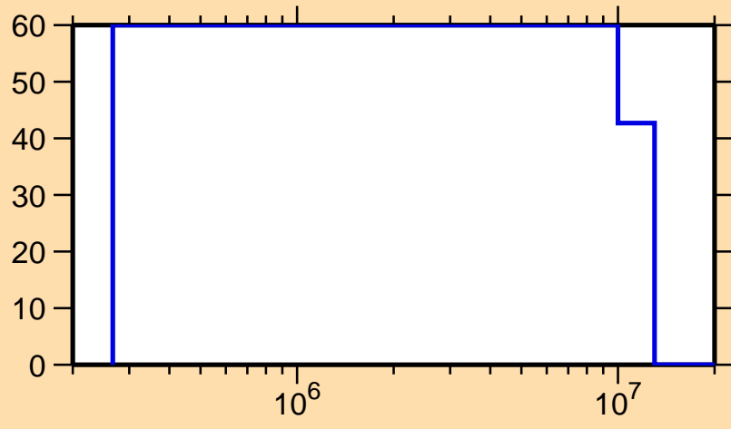
\Delta\sigma/\sigma vs. E for ^{258}_{1}
