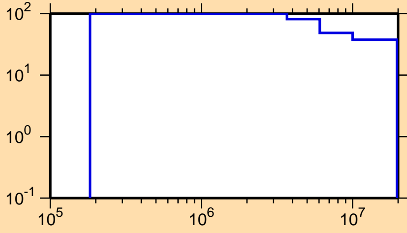
\Delta\sigma/\sigma vs. E for ^{258}\text{Po}
