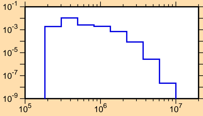
\sigma vs. E for ^{258}_{1}
