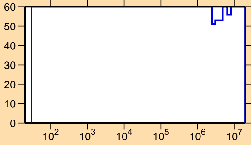
\Delta\sigma/\sigma vs. E for ^{258}\text{Ge}
