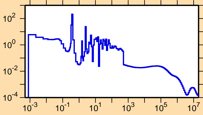
\sigma vs. E for ^{258}\gamma
