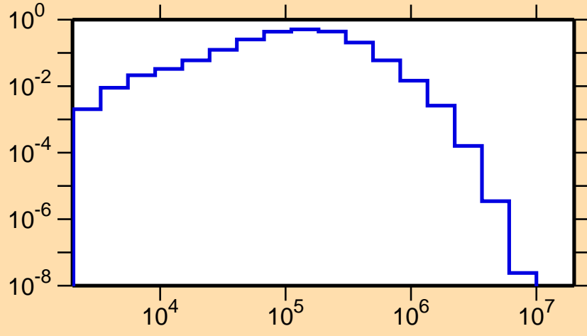
\sigma vs. E for ^{258}_{2}
