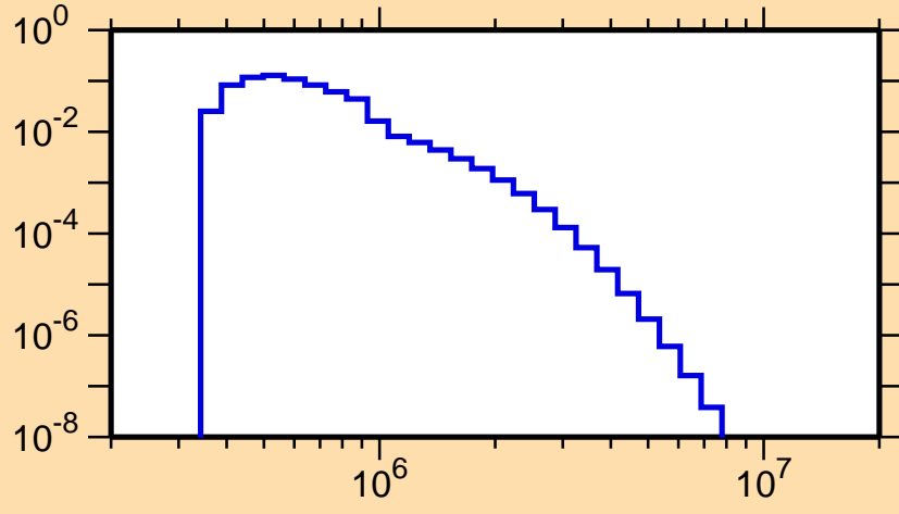
\sigma vs. E for ^{260}_{2}
