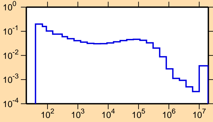
\sigma vs. E for ^{260}\alpha
