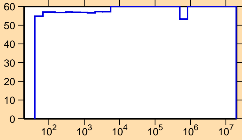
\Delta\sigma/\sigma vs. E for ^{260}\gamma
