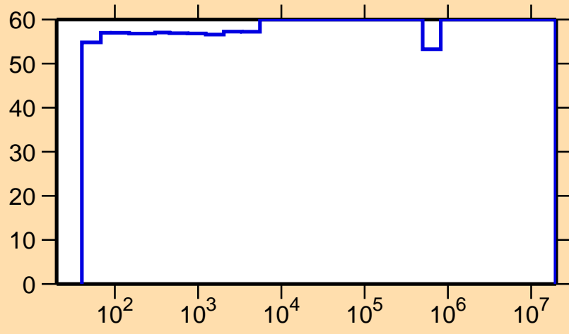
\Delta\sigma/\sigma vs. E for ^{260}\gamma
