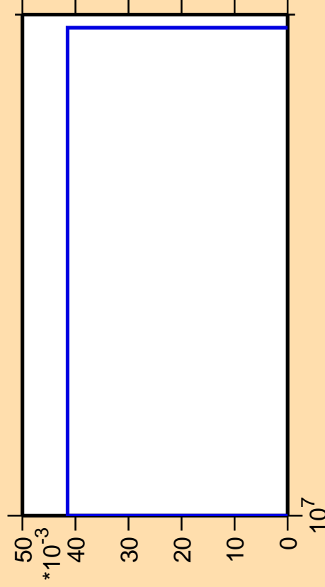
\Delta\sigma/\sigma vs. E for ^{260}
