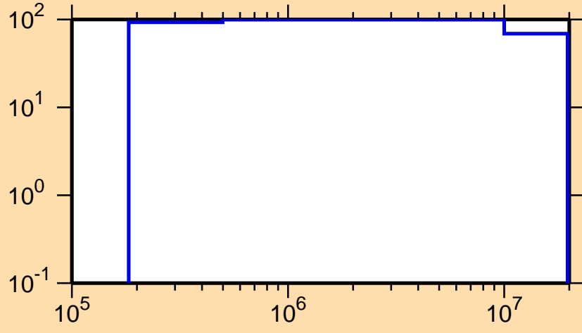
\Delta\sigma/\sigma vs. E for ^{260}_{1}
