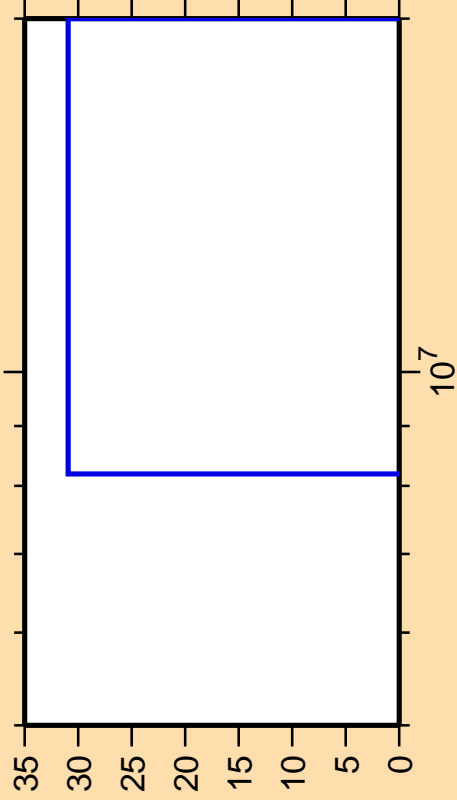
\Delta\sigma/\sigma vs. E for ^{260}\text{He3}
