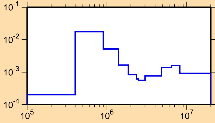
\sigma vs. E for ^{260}_{4}
