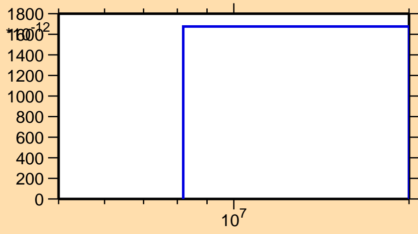
\sigma vs. E for ^{260}\text{He3}
