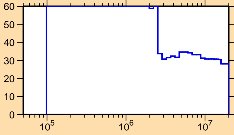
\Delta\sigma/\sigma vs. E for ^{261}_{1}\text{Po}
