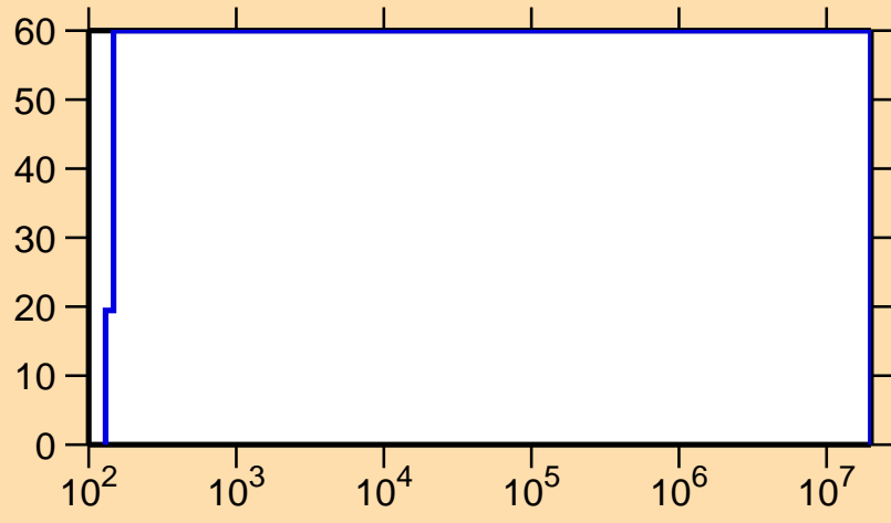
\Delta\sigma/\sigma vs. E for ^{262}\gamma
