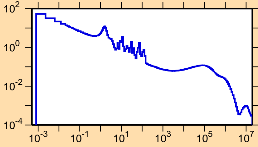
\sigma vs. E for ^{262}\text{Pu}
