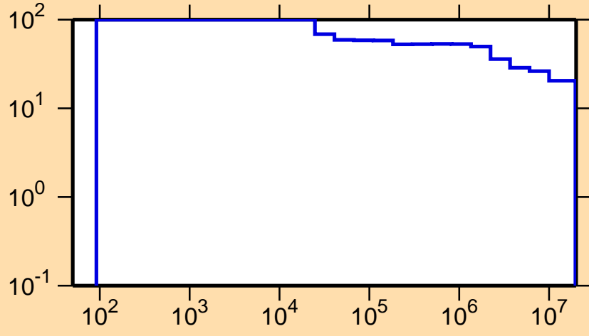
\Delta\sigma/\sigma vs. E for ^{262}
