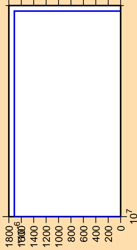
\Delta\sigma/\sigma vs. E for ^{262}
