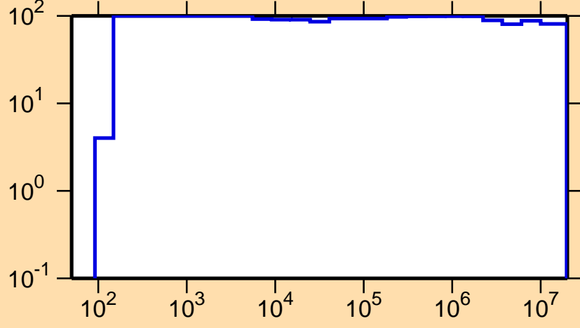
\Delta\sigma/\sigma vs. E for ^{262}\gamma
