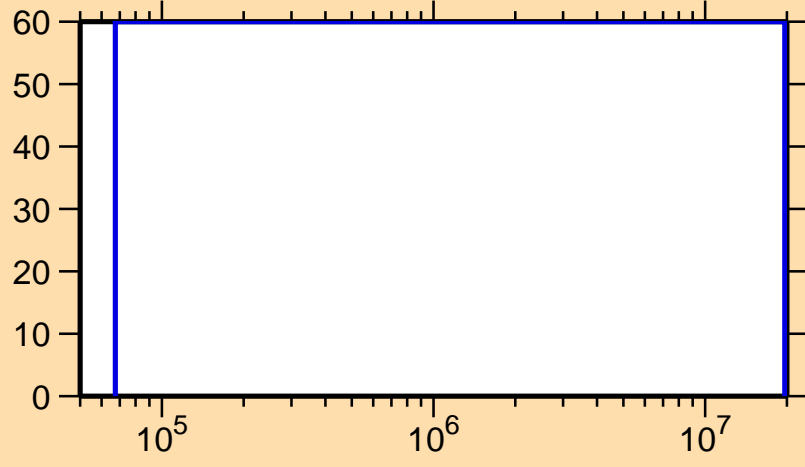
\Delta\sigma/\sigma vs. E for ^{262}_{1}
