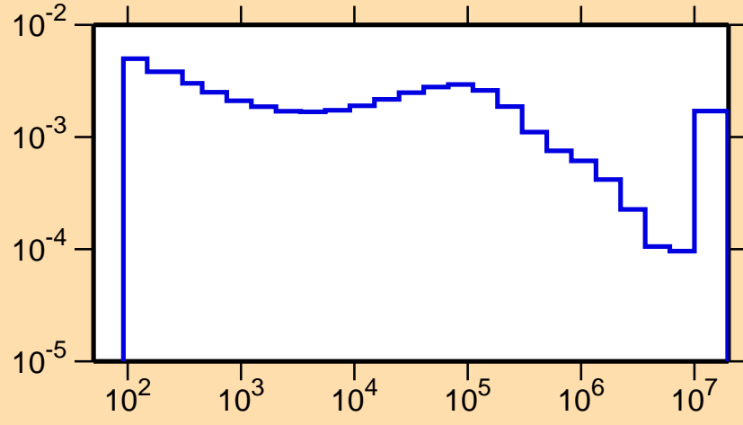
\sigma vs. E for ^{262}\alpha
