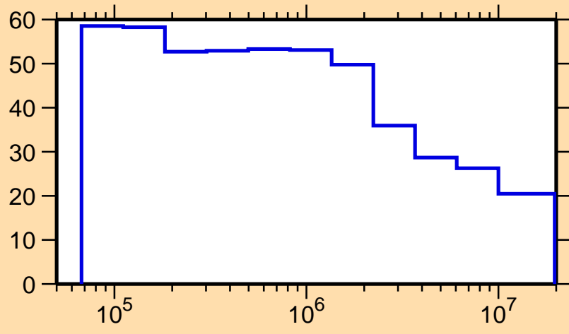
\Delta\sigma/\sigma vs. E for ^{262}
