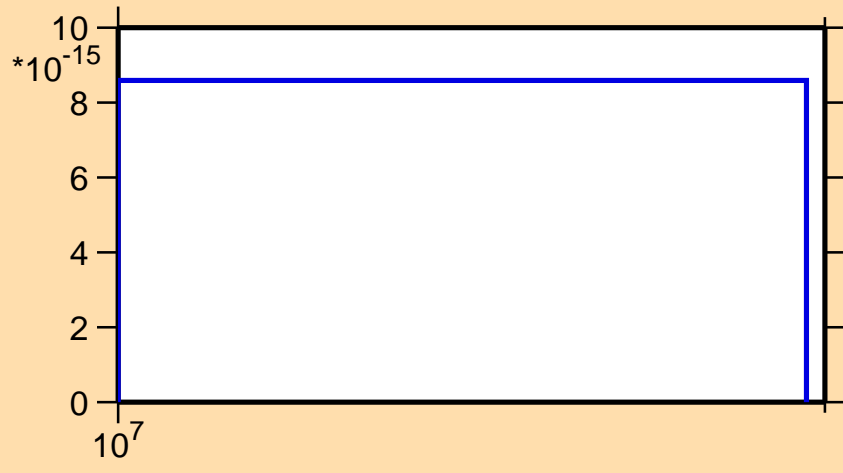
\sigma vs. E for ^{262}
