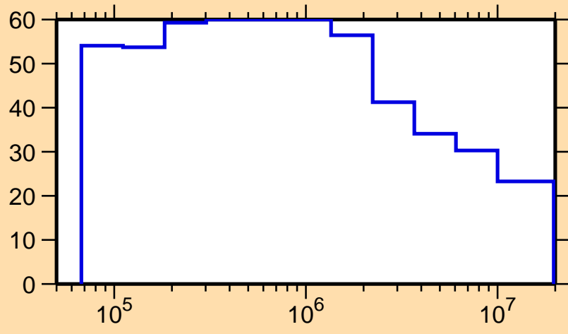
Δσ/σ vs. E for 262
