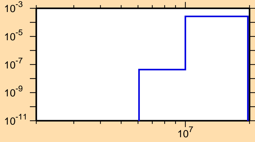
\sigma vs. E for ^{262}
