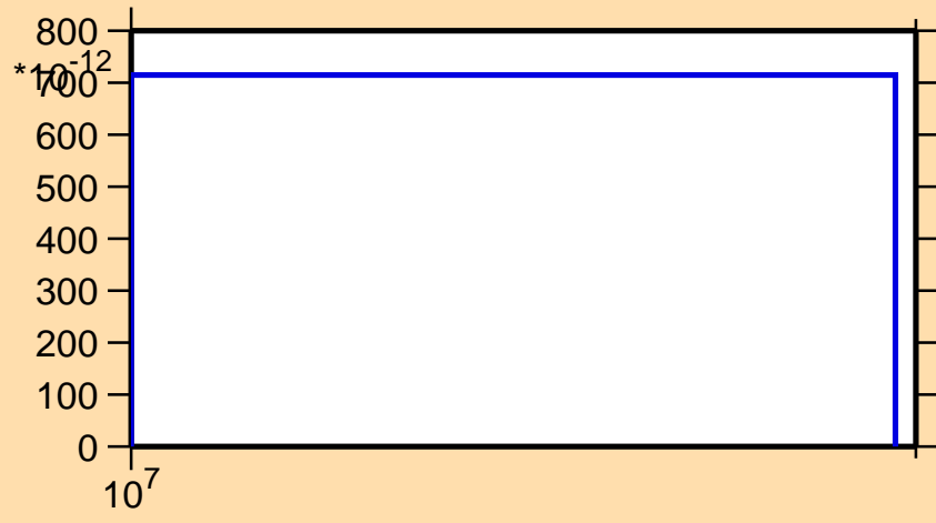
\sigma vs. E for ^{262}\text{He3} )
