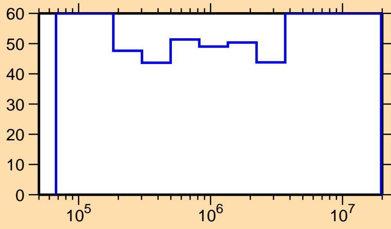
Δσ/σ vs. E for 263
