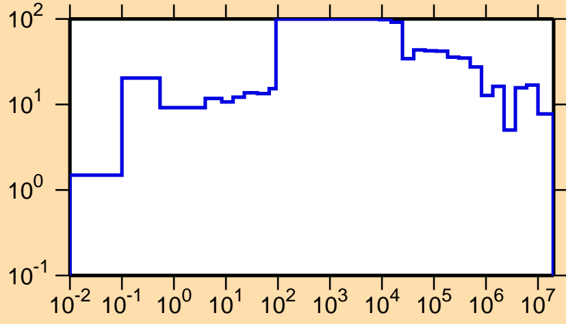
\Delta\sigma/\sigma vs. E for ^{263}\text{Pa}
