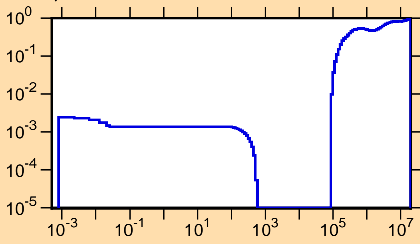
\mu vs. E for ^{264}
