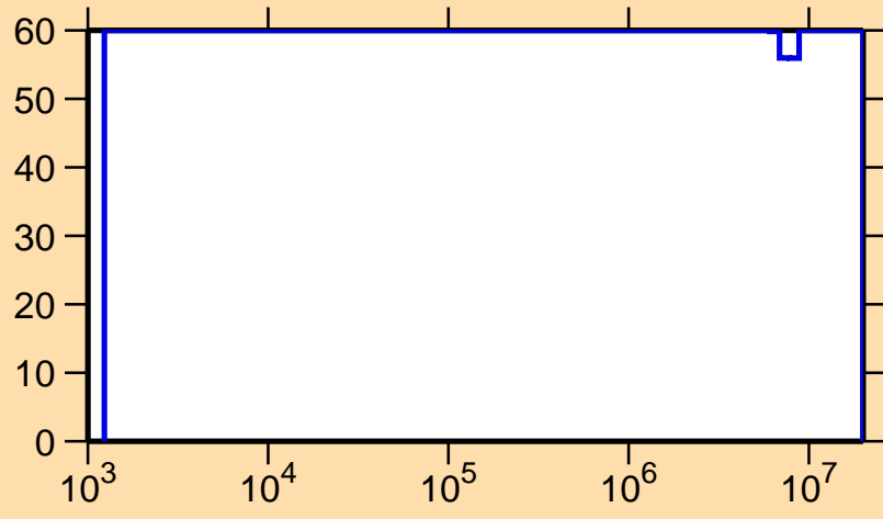
\Delta\sigma/\sigma vs. E for ^{264}\gamma
