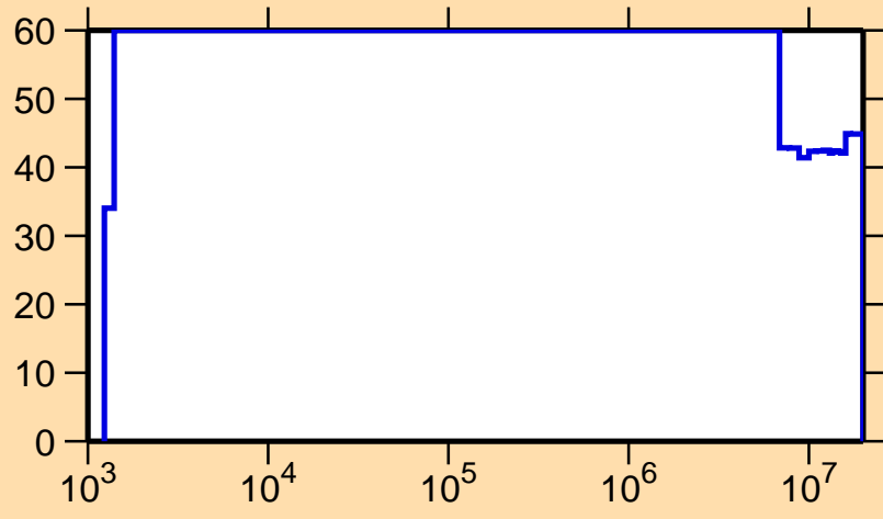
\Delta\sigma/\sigma vs. E for ^{266}\gamma
