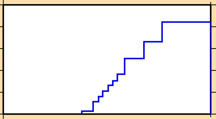
\sigma vs. E for ^{268}\text{He3}
