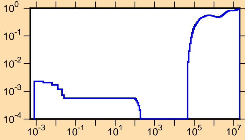
\mu vs. E for ^{280}
