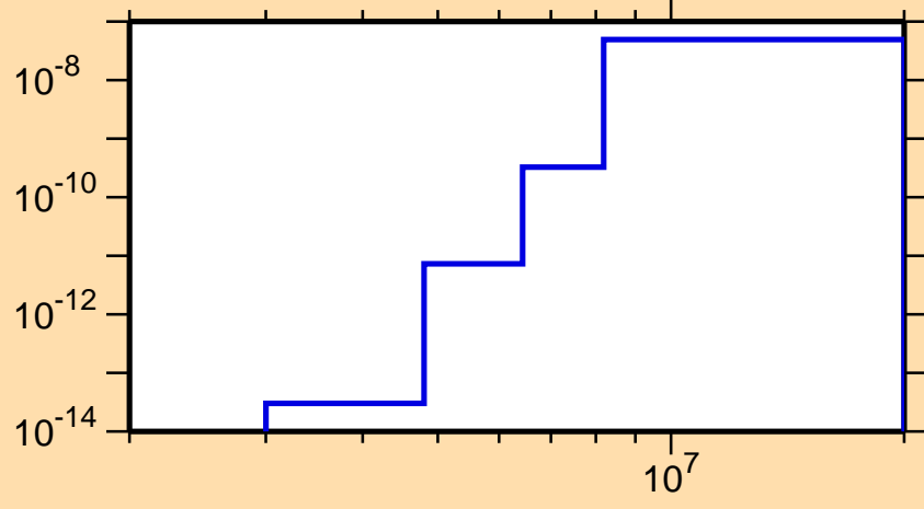
\sigma vs. E for ^{280}\alpha
