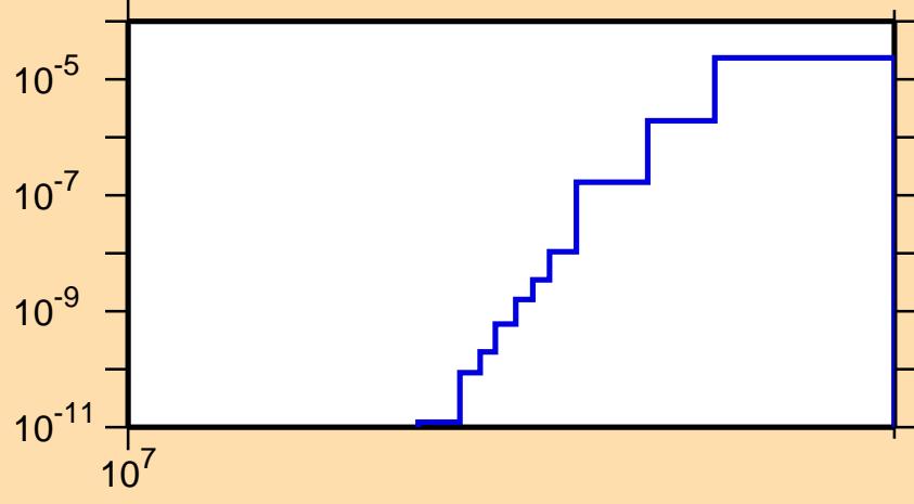
\sigma vs. E for ^{142}\text{Dy}(n,pt)
