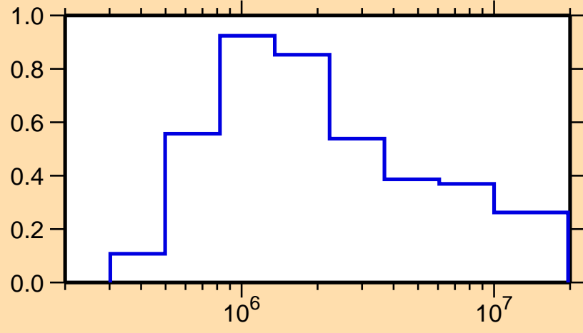
\sigma vs. E for ^{142}\text{Dy}(n,\text{inel.})
