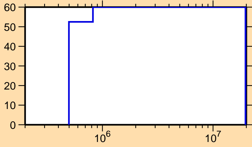
\Delta\sigma/\sigma vs. E for ^{142}\text{Dy}(n,n\text{cont.})
