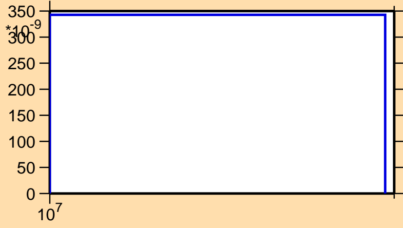
\sigma vs. E for ^{142}\text{Dy}(n,\text{pt})
