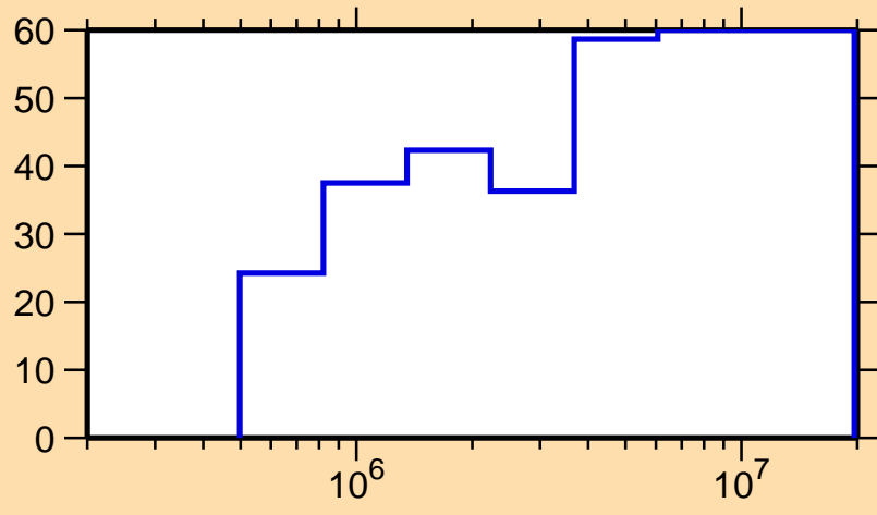
\Delta\sigma/\sigma vs. E for ^{142}\text{Dy}(n,el.)
