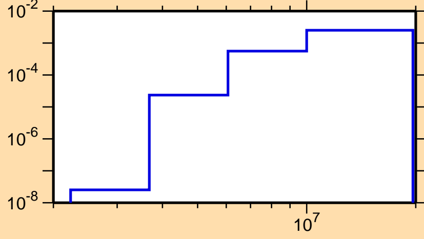
\sigma vs. E for ^{142}\text{Dy}(n,n\alpha)
