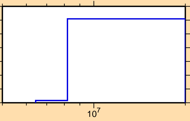
\sigma vs. E for ^{142}\text{Dy}(\text{mt117})
