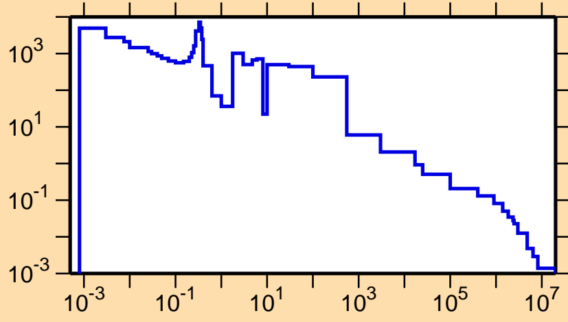
\sigma vs. E for ^{142}\text{Dy}(n,\gamma)
