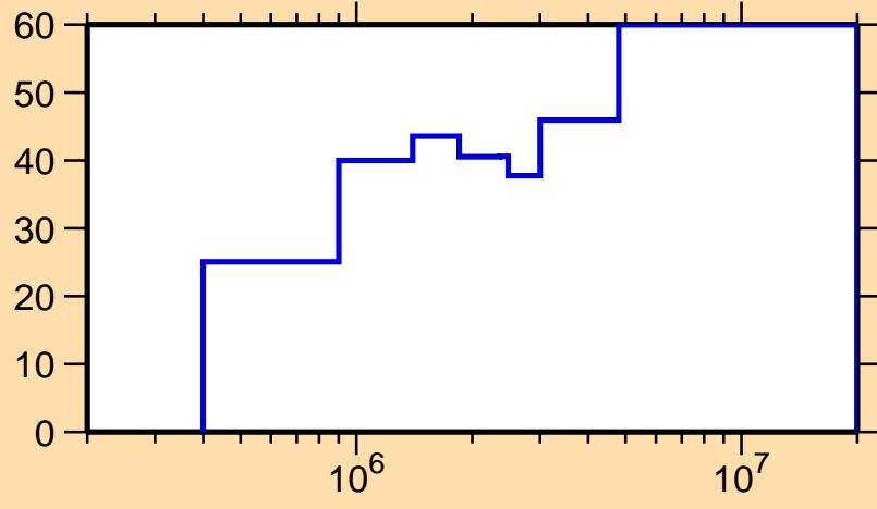
\Delta\sigma/\sigma vs. E for ^{142}\text{Dy}(n,el.)
