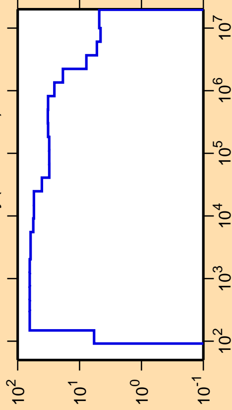
\Delta\sigma/\sigma vs. E for ^{143}\text{Dy}(n,\text{nonel.})
