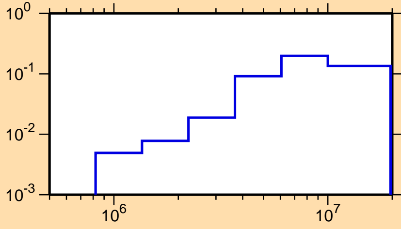
\sigma vs. E for ^{143}\text{Dy}(n,n\text{cont.})
