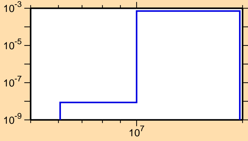
\sigma vs. E for ^{143}\text{Dy}(n,pd)
