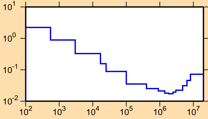
\sigma vs. E for ^{143}\text{Dy}(n,\alpha)
