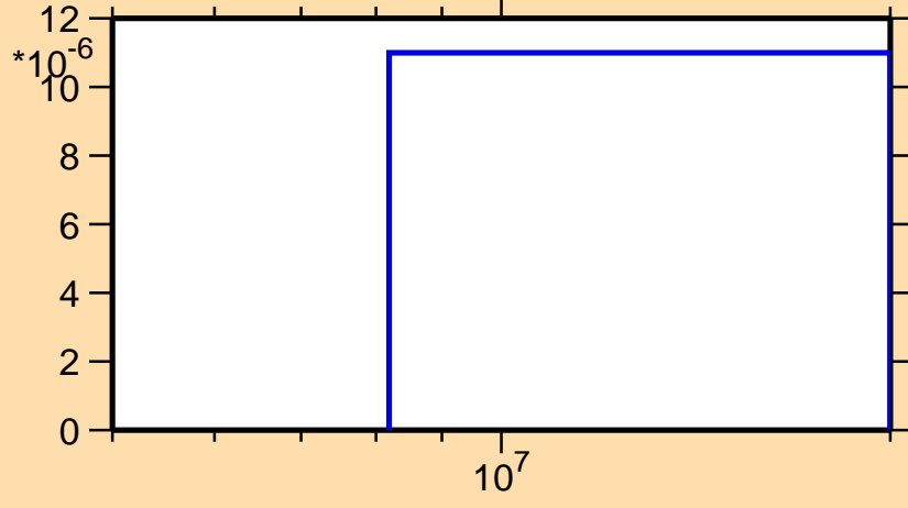
\sigma vs. E for ^{143}\text{Dy}(n,\text{pt})
