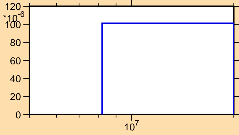
\sigma vs. E for ^{143}\text{Dy}(n,t)
