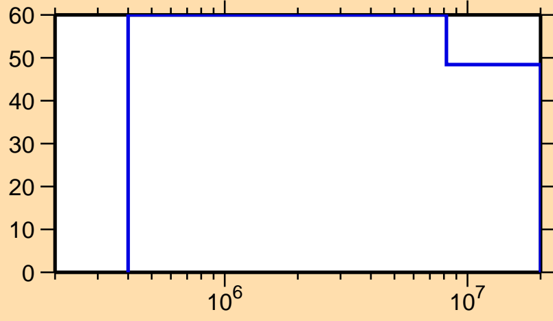
\Delta\sigma/\sigma vs. E for ^{143}\text{Dy}(n,n\text{cont.})
