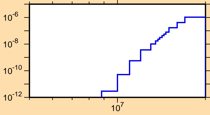
\sigma vs. E for ^{143}\text{Dy}(\text{mt117})
