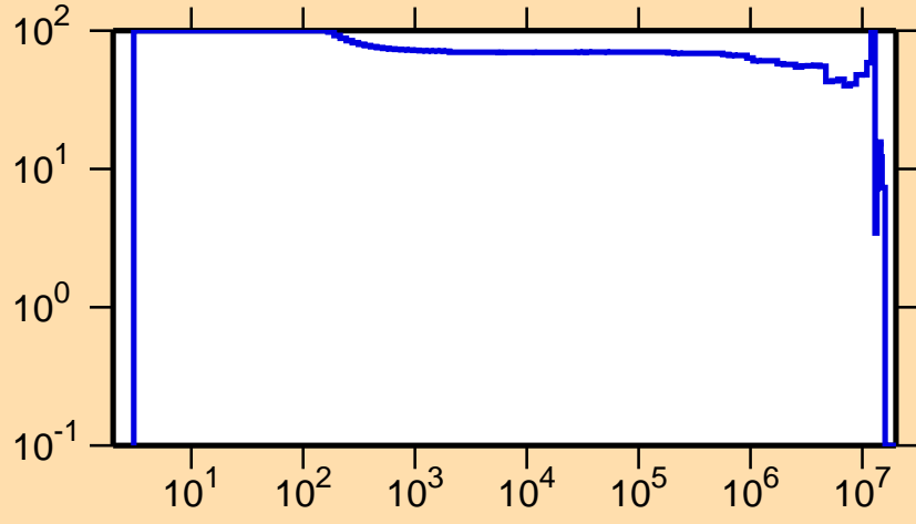
\Delta\sigma/\sigma vs. E for ^{143}\text{Dy}(n,n_1)
