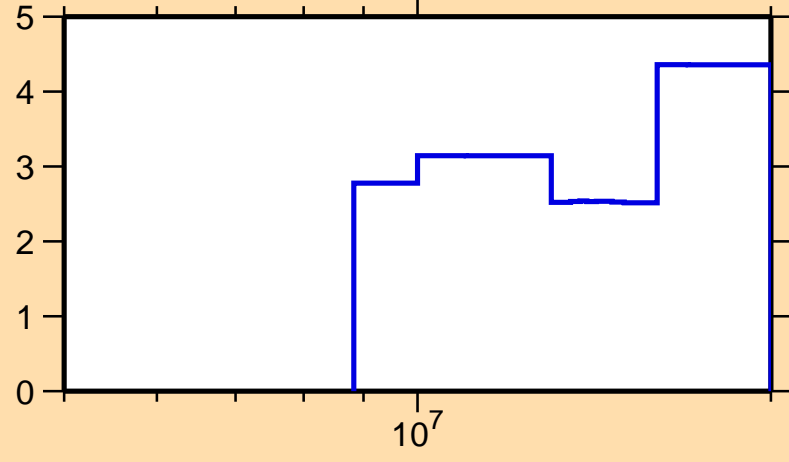
\Delta\sigma/\sigma vs. E for ^{143}\text{Dy}(n,\text{tot.})
