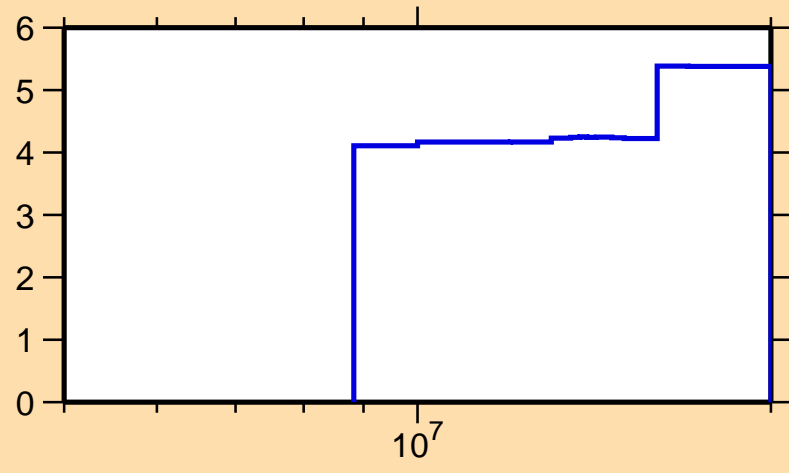
\Delta\sigma/\sigma vs. E for ^{143}\text{Dy}(n,\text{nonel.})
