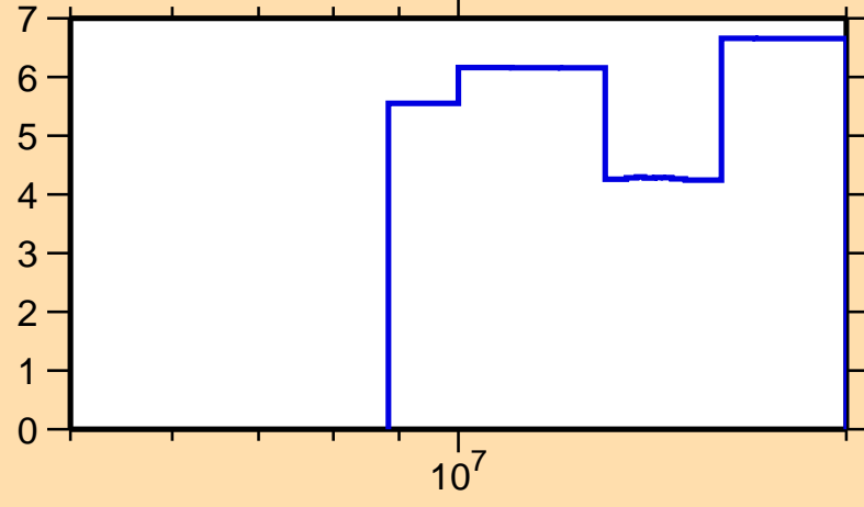
\Delta\sigma/\sigma vs. E for ^{143}\text{Dy}(n,\text{el.})
