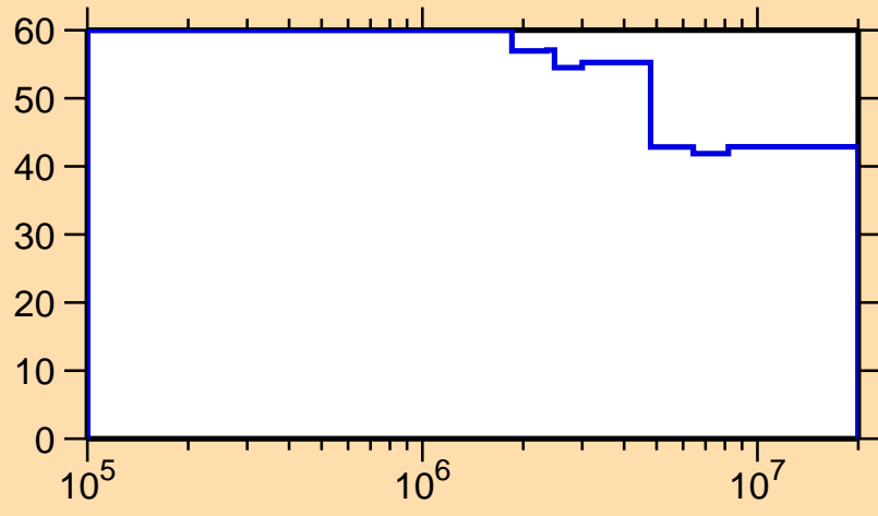
\Delta\sigma/\sigma vs. E for ^{143}\text{Dy}(n,n_1)
