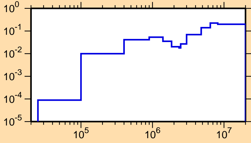
\sigma vs. E for ^{143}\text{Dy}(n,\text{inel.})
