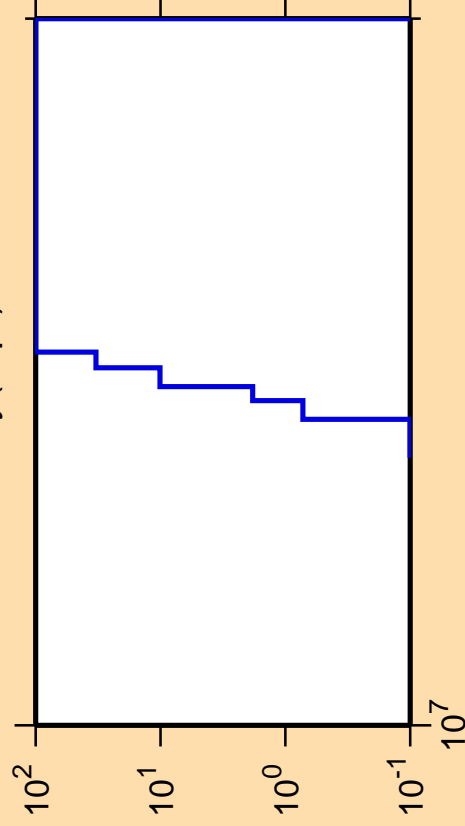
\Delta\sigma/\sigma vs. E for ^{144}\text{Dy}(n,pt)
