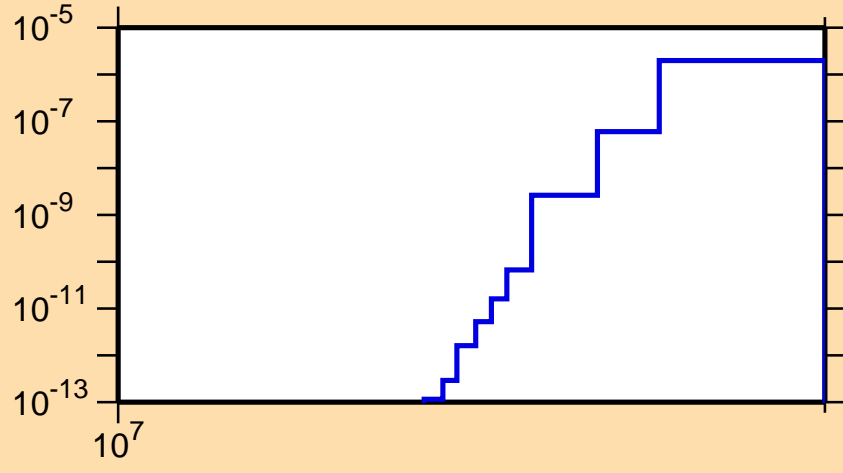
\sigma vs. E for ^{144}\text{Dy}(n,pt)
