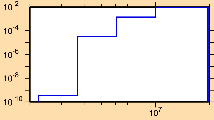
\sigma vs. E for ^{144}\text{Dy}(n,n\alpha)
