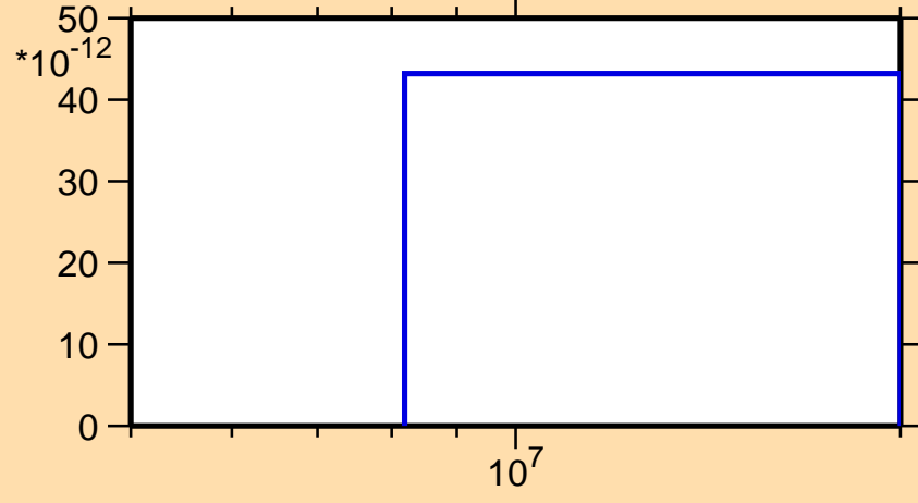
\sigma vs. E for ^{144}\text{Dy}(n,nd)
