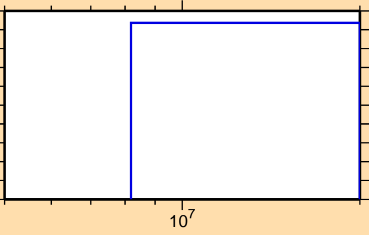
\sigma vs. E for ^{144}\text{Dy}(n,t)
