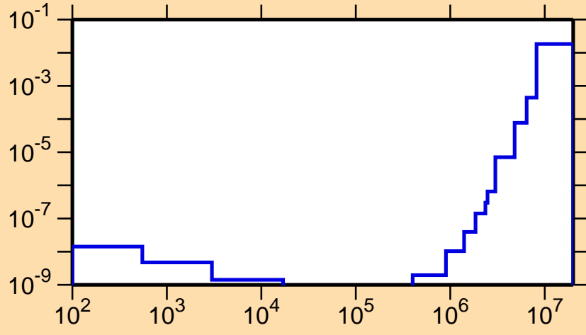
\sigma vs. E for ^{144}\text{Dy}(n,p\alpha)
