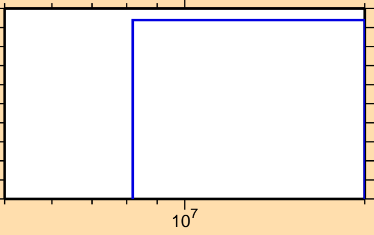
\sigma vs. E for ^{144}\text{Dy}(n,\text{pt})
