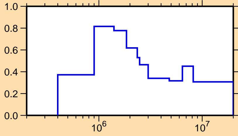
\sigma vs. E for ^{144}\text{Dy}(n,\text{inel.})
