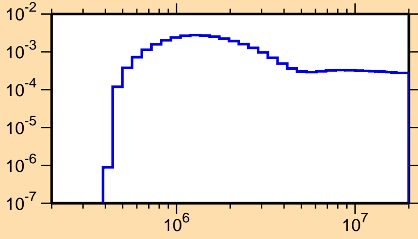
\sigma vs. E for ^{145}\text{Dy}(n,n_4)
