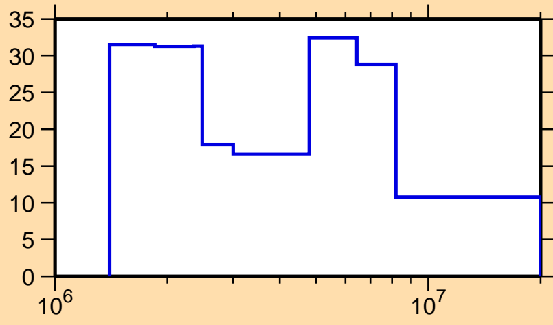
\Delta\sigma/\sigma vs. E for ^{145}\text{Dy}(n,el.)
