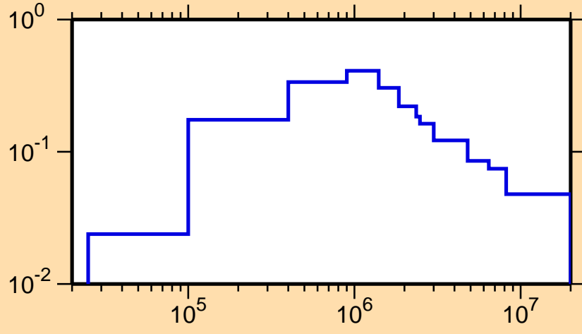
\sigma vs. E for ^{145}\text{Dy}(n,n_1)
