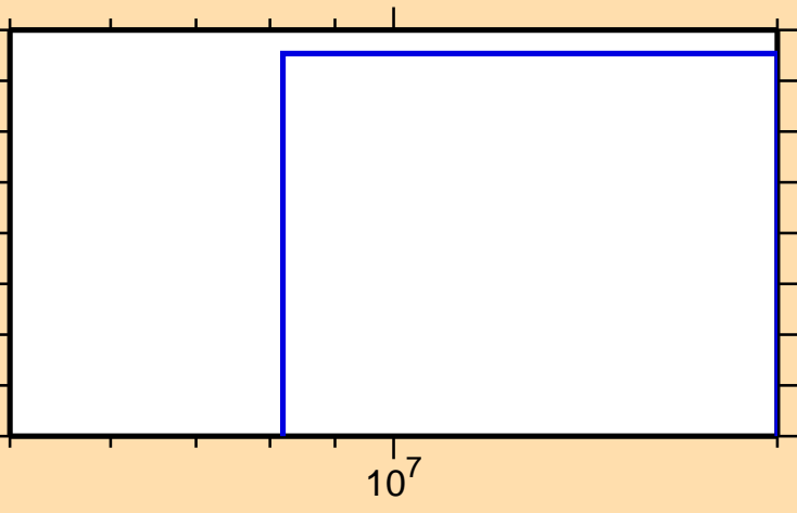
\sigma vs. E for ^{145}\text{Dy}(n,2np)
