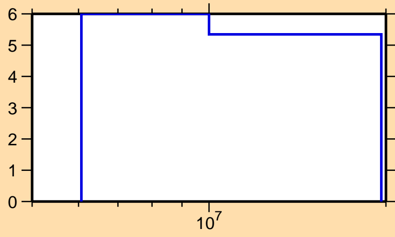
\Delta\sigma/\sigma vs. E for ^{145}\text{Dy}(n,\text{nonel.})
