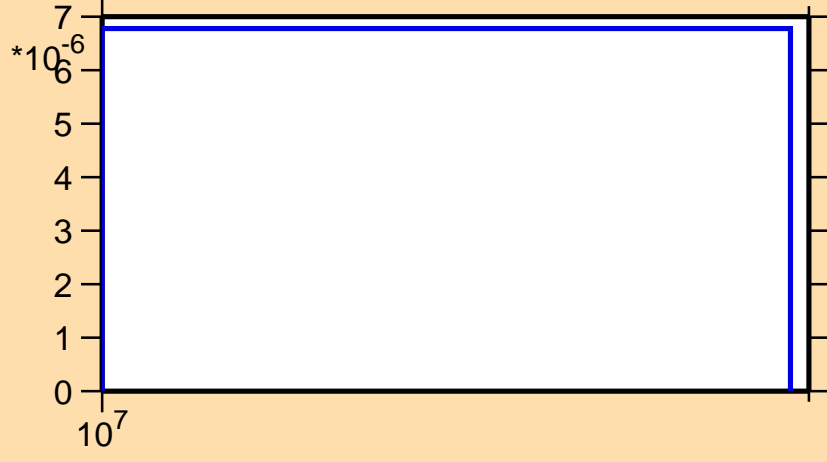
\sigma vs. E for ^{145}\text{Dy}(n,2np)
