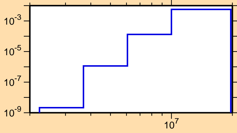
\sigma vs. E for ^{145}\text{Dy}(n,n\alpha)
