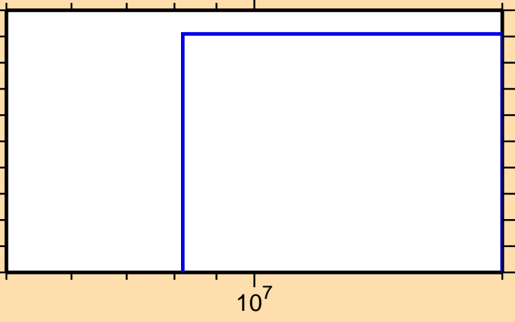
\sigma vs. E for ^{145}\text{Dy}(n,nd)
