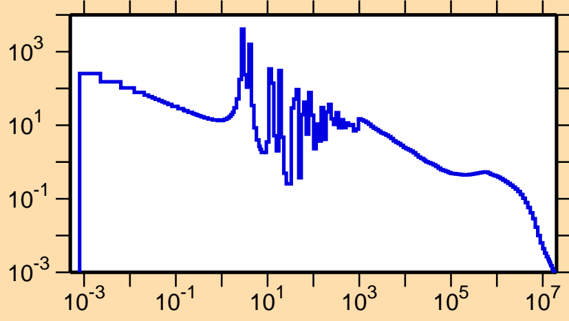
\sigma vs. E for ^{146}\text{Dy}(n,\gamma)
