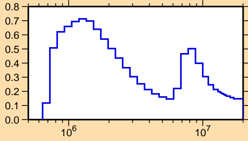
\sigma vs. E for ^{146}\text{Dy}(n,\text{inel.})
