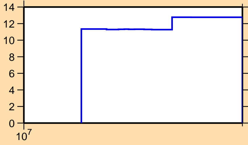
\Delta\sigma/\sigma vs. E for ^{146}\text{Dy}(n,\text{nonel.})
