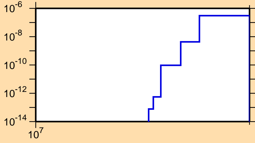
\sigma vs. E for ^{146}\text{Dy}(n,2n\alpha)
