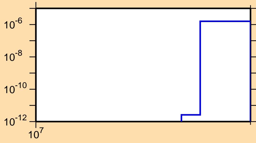
\sigma vs. E for ^{146}\text{Dy}(n,2np)
