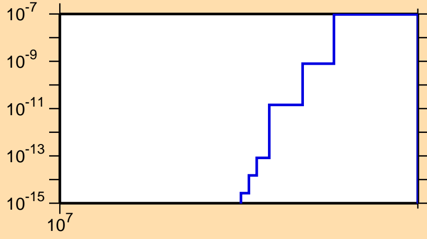
\sigma vs. E for ^{146}\text{Dy}(n,\text{pt})
