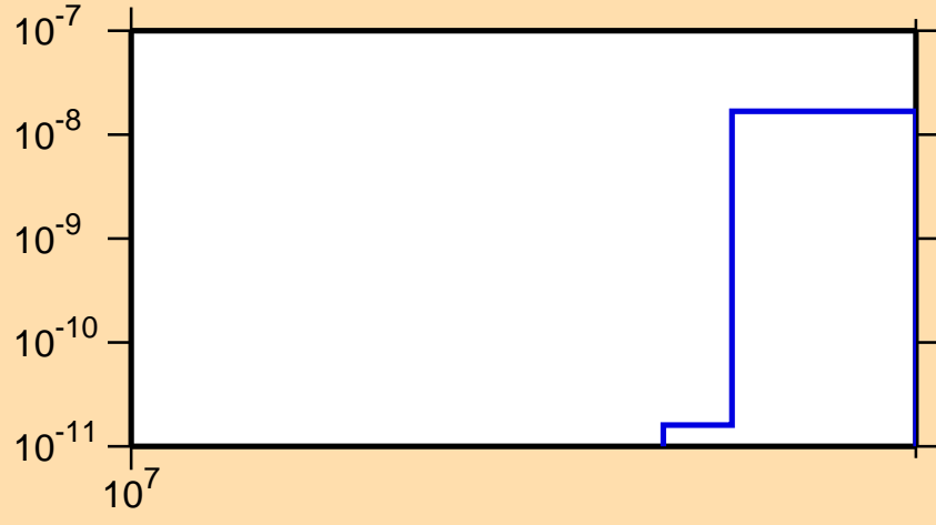
\sigma vs. E for ^{146}\text{Dy}(n,nd)
