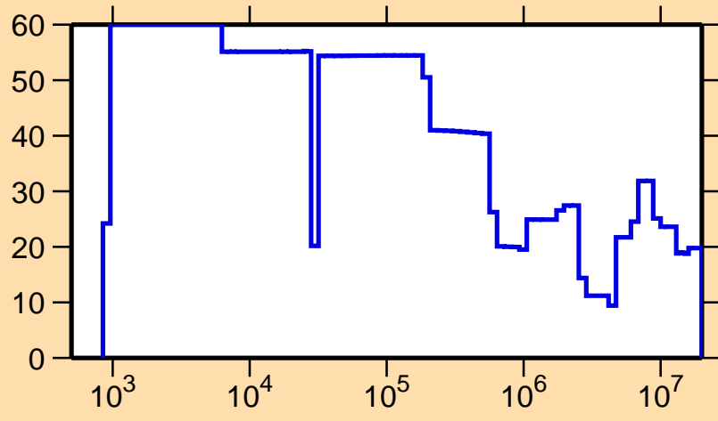
\Delta\sigma/\sigma vs. E for ^{146}\text{Dy}(n,\text{tot.})
