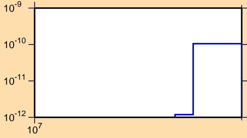
\sigma vs. E for ^{146}\text{Dy} (mt 34)
