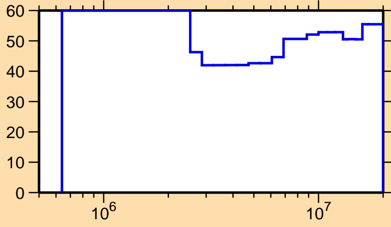
\Delta\sigma/\sigma vs. E for ^{146}\text{Dy}(n,n_1)
