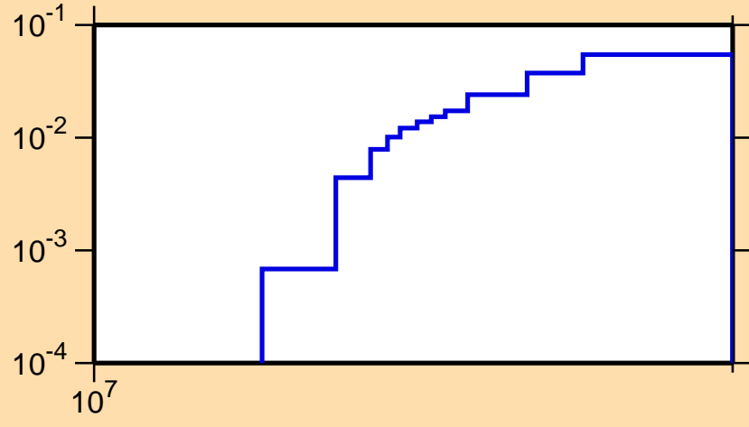
\sigma vs. E for ^{146}\text{Dy}(n,2n)
