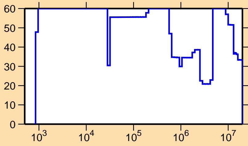
\Delta\sigma/\sigma vs. E for ^{146}\text{Dy}(n,\text{el.})
