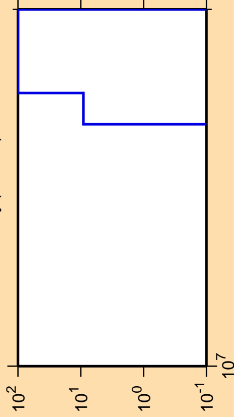
\Delta\sigma/\sigma vs. E for ^{146}\text{Dy} (mt 34)
