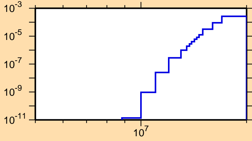
\sigma vs. E for ^{146}\text{Dy}(n,\text{pd})
