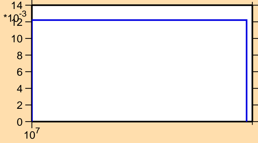
\sigma vs. E for ^{146}\text{Dy}(n,2n)
