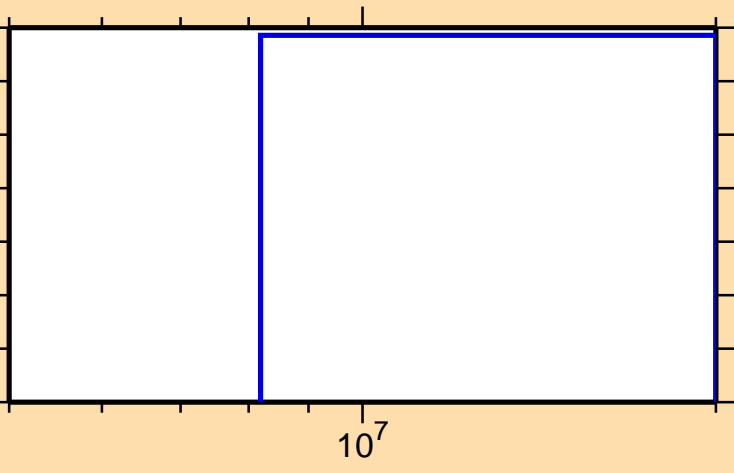
\sigma vs. E for ^{146}\text{Dy}(n,nd)
