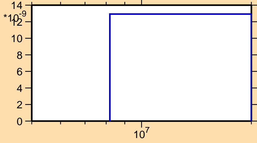
\sigma vs. E for ^{146}\text{Dy}(n,2np)
