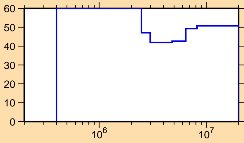
\Delta\sigma/\sigma vs. E for ^{146}\text{Dy}(n,n_1)
