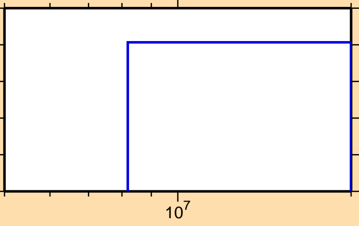
\sigma vs. E for ^{146}\text{Dy} (mt 45)
