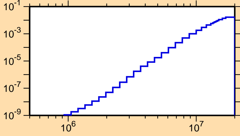
\sigma vs. E for ^{147}\text{Dy}(n,p\alpha)
