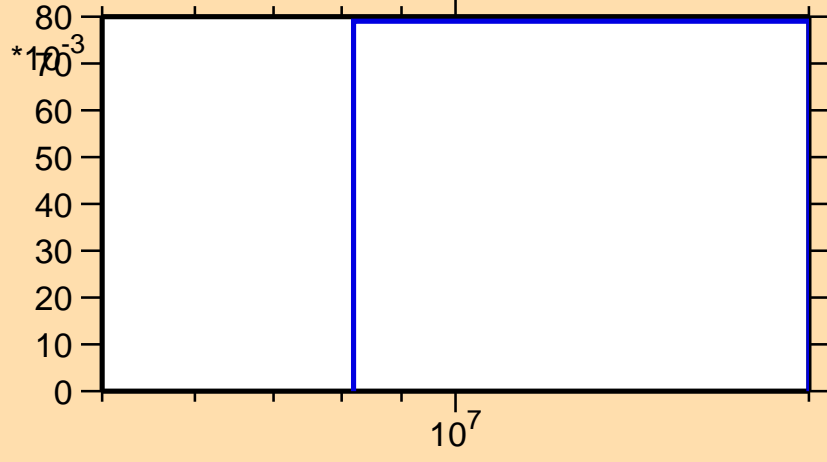
\sigma vs. E for ^{147}\text{Dy}(n,2n)
