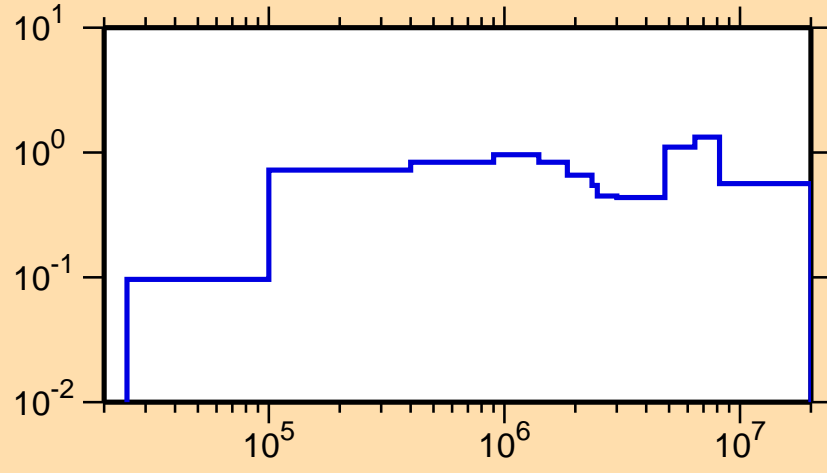
\sigma vs. E for ^{147}\text{Dy}(n,\text{inel.})
