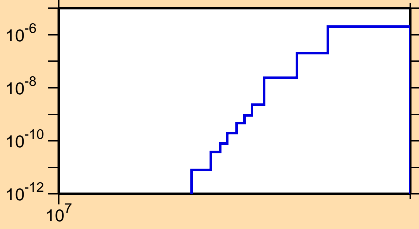
\sigma vs. E for ^{147}\text{Dy}(n,pt)
