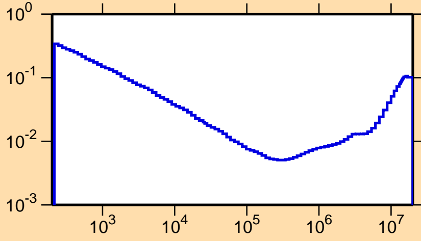
\sigma vs. E for ^{147}\text{Dy}(n,\alpha)
