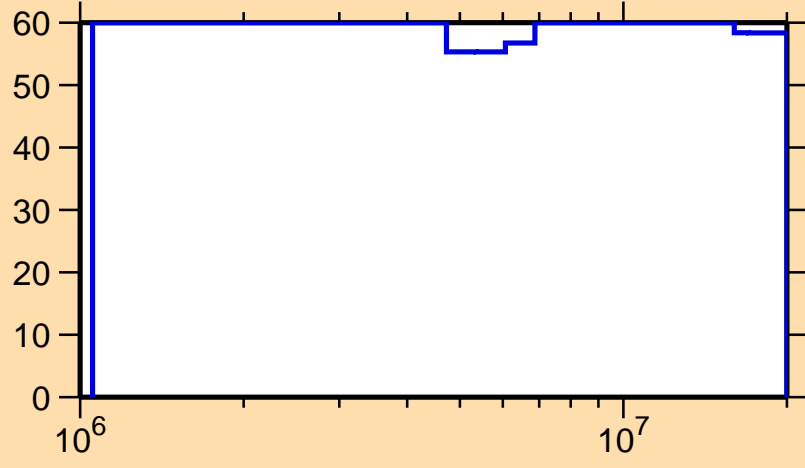
\Delta\sigma/\sigma vs. E for ^{147}\text{Dy}(n,n\text{cont.})
