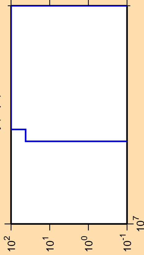
\Delta\sigma/\sigma vs. E for ^{147}\text{Dy}(n,pt)
