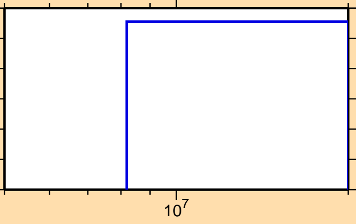
\sigma vs. E for ^{147}\text{Dy}(n,\text{pt})
