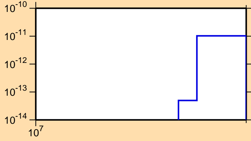
\sigma vs. E for ^{148}\text{Dy} (mt 34)
