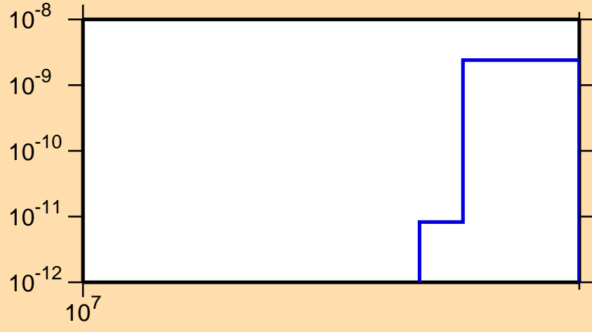
\sigma vs. E for ^{148}\text{Dy}(n,\text{pt})
