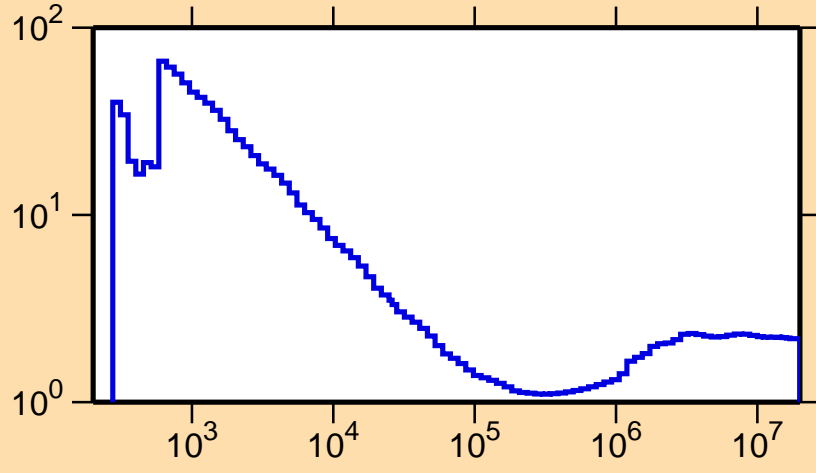
\sigma vs. E for ^{149}\text{Dy}(n,\text{nonel.})
