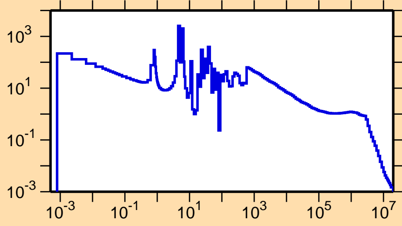
\sigma vs. E for ^{149}\text{Dy}(n,\gamma)
