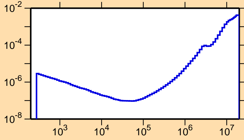
\sigma vs. E for ^{149}\text{Dy}(n,p\alpha)
