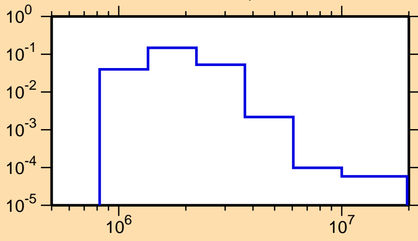
\sigma vs. E for ^{149}\text{Dy}(n,n_1)
