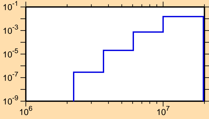
\sigma vs. E for ^{149}\text{Dy}(n,n\alpha)
