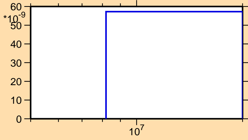
\sigma vs. E for ^{149}\text{Dy}(n,\text{pt})
