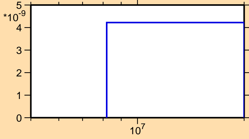
\sigma vs. E for ^{149}\text{Dy}(\text{mt117})
