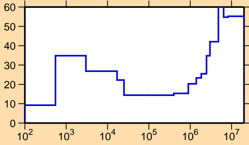
\Delta\sigma/\sigma vs. E for ^{149}\text{Dy}(n,\gamma)
