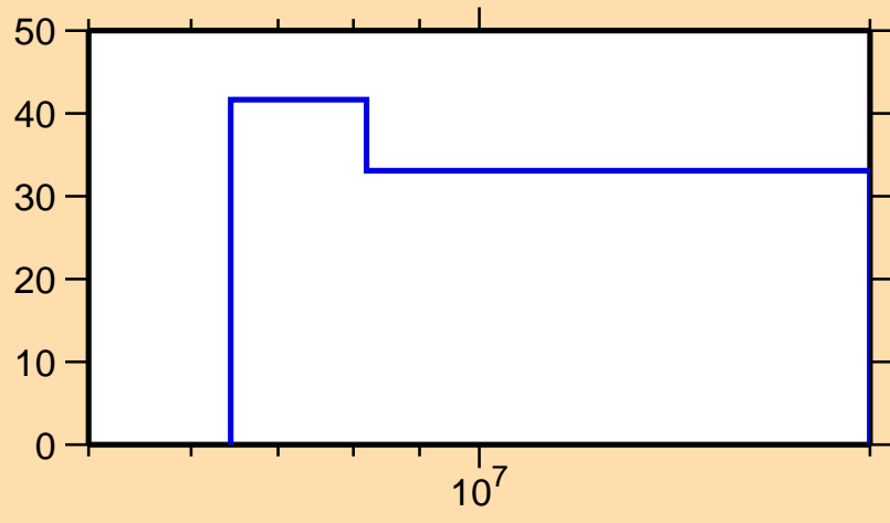
\Delta\sigma/\sigma vs. E for ^{149}\text{Dy}(n,2n)
