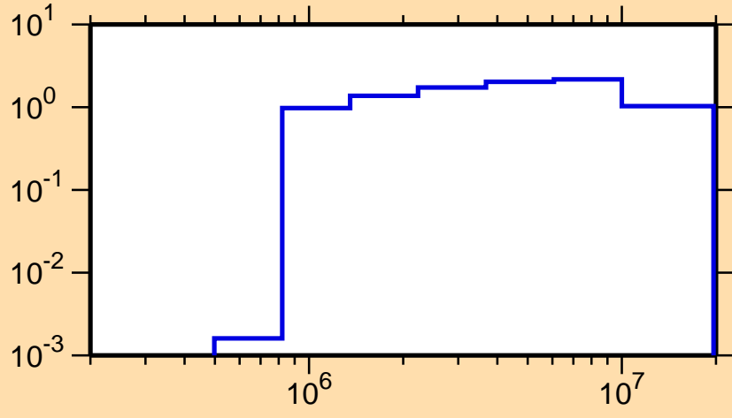
\sigma vs. E for ^{150}\text{Dy}(n,\text{inel.})
