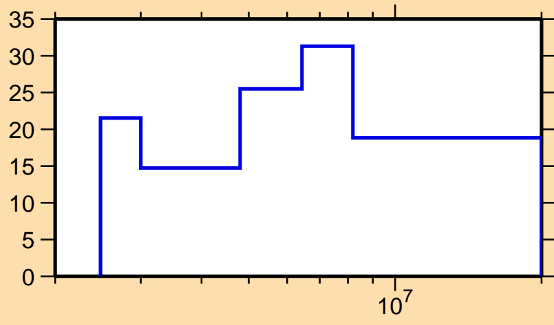
\Delta\sigma/\sigma vs. E for ^{150}\text{Dy}(n,inel.)
