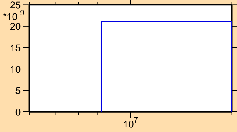
\sigma vs. E for ^{150}\text{Dy}(n,nd)
