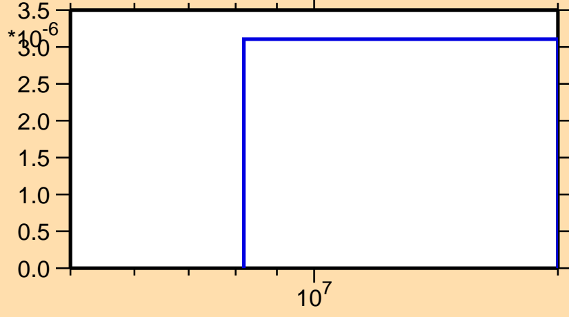
\sigma vs. E for ^{150}\text{Dy}(n,2n\alpha)
