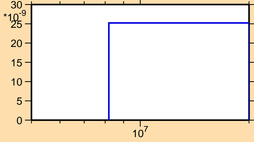
\sigma vs. E for ^{150}\text{Dy}(n,pd)
