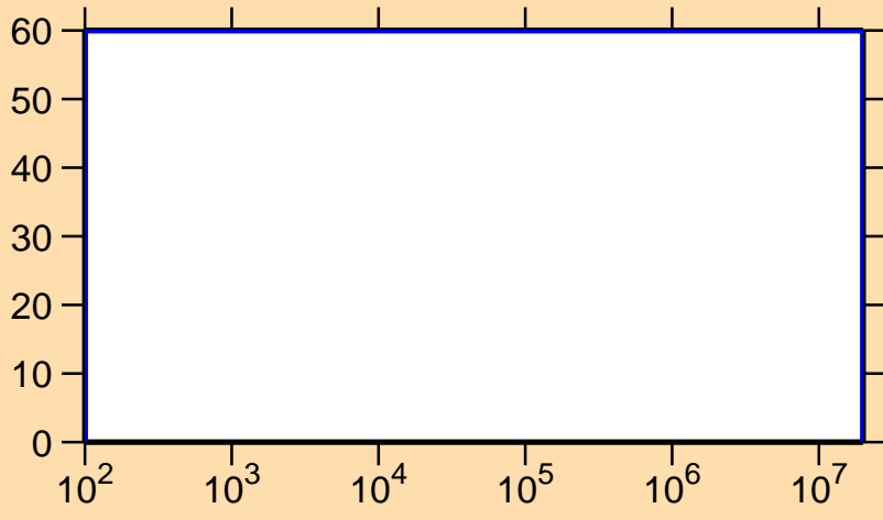
\Delta\sigma/\sigma vs. E for ^{150}\text{Dy}(n,\gamma)
