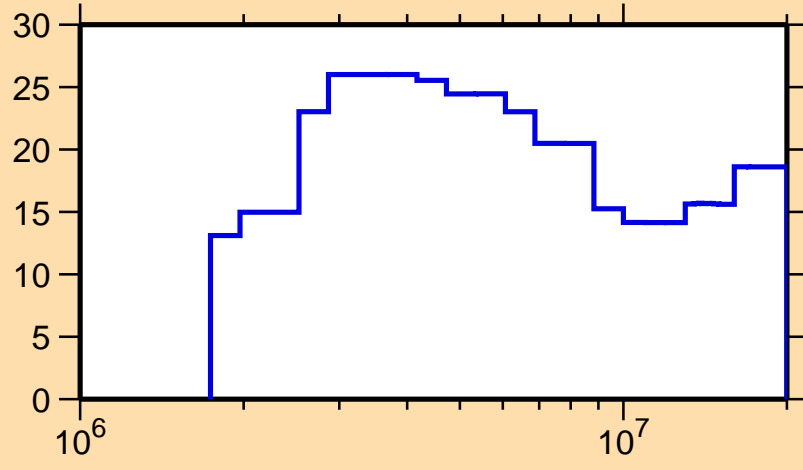
\Delta\sigma/\sigma vs. E for ^{151}\text{Dy}(n,el.)
