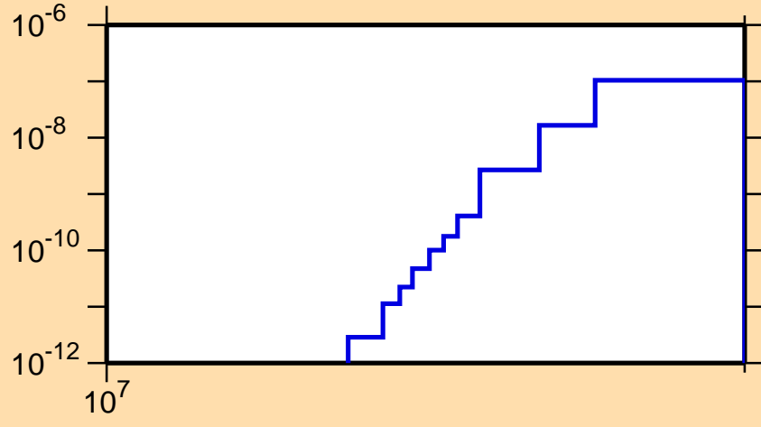
\sigma vs. E for ^{151}\text{Dy}(n,pd)
