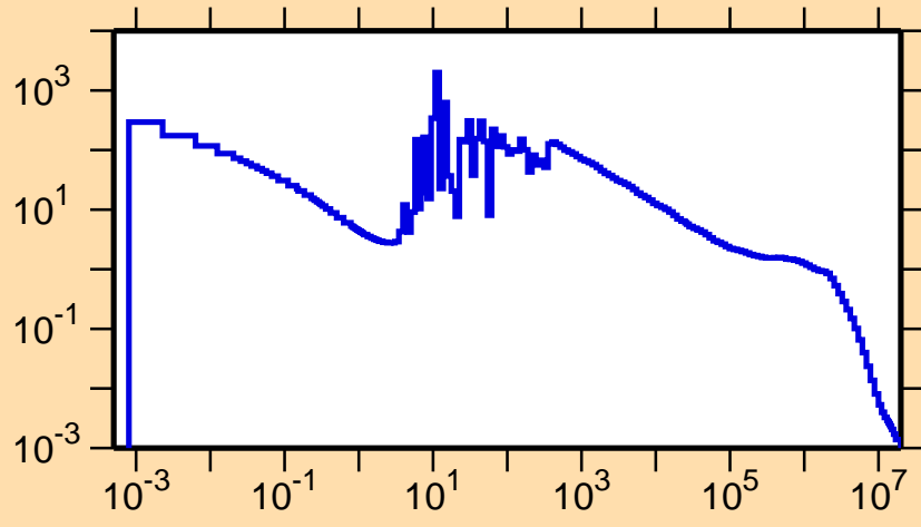
\sigma vs. E for ^{151}\text{Dy}(n,\gamma)
