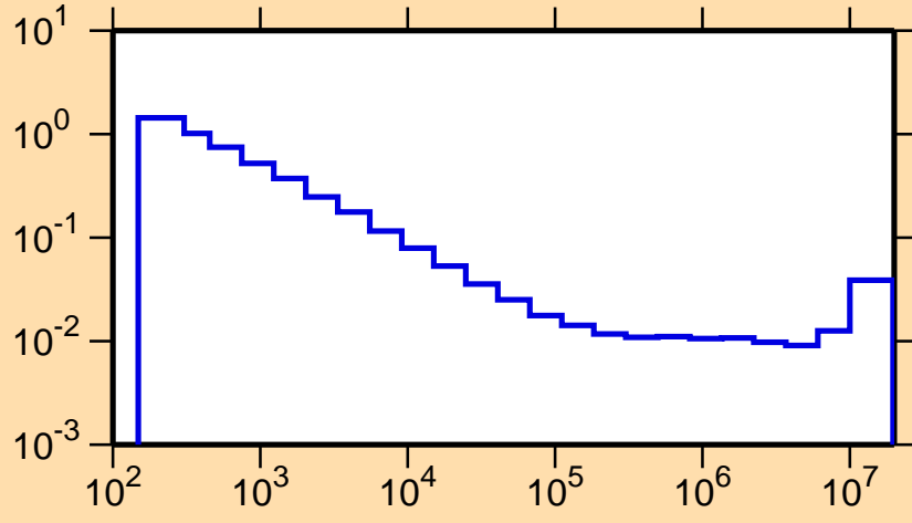
\sigma vs. E for ^{151}\text{Dy}(n,\alpha)
