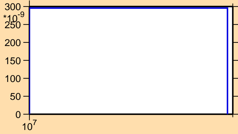
\sigma vs. E for ^{151}\text{Dy}(n,\text{nd})
