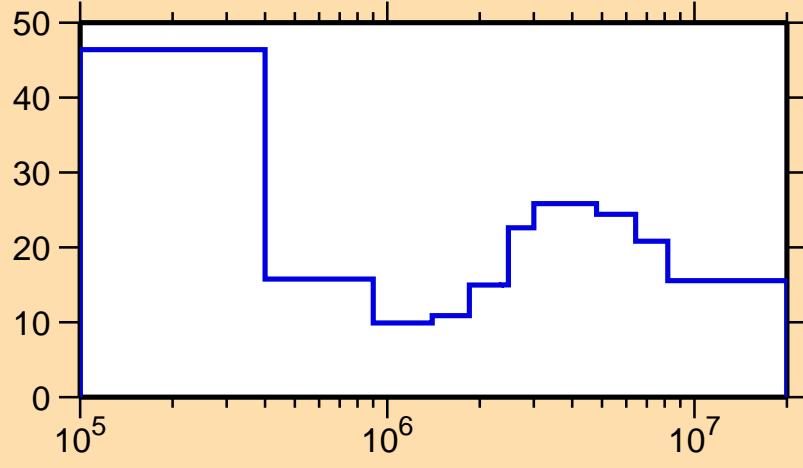
\Delta\sigma/\sigma vs. E for ^{151}\text{Dy}(n,\text{el.})
