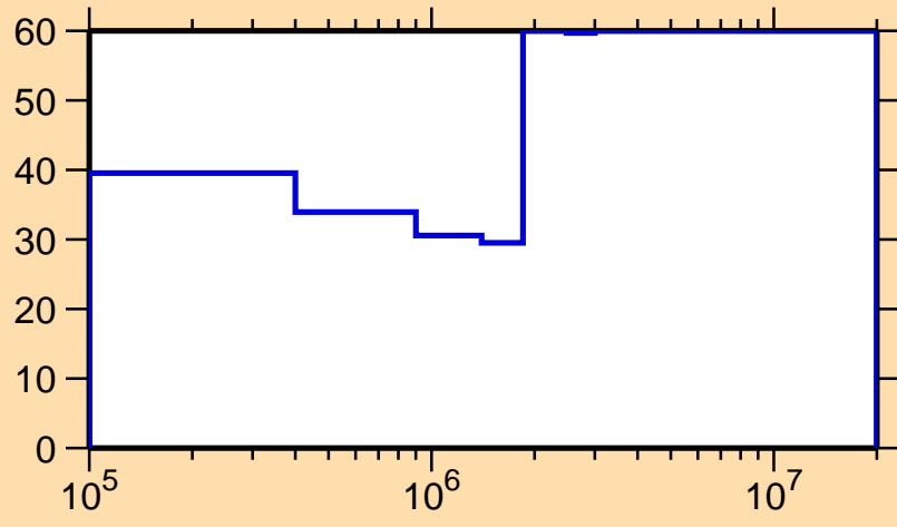
\Delta\sigma/\sigma vs. E for ^{151}\text{Dy}(n,n_1)
