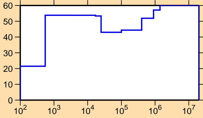
\Delta\sigma/\sigma vs. E for ^{151}\text{Dy}(n,\gamma)
