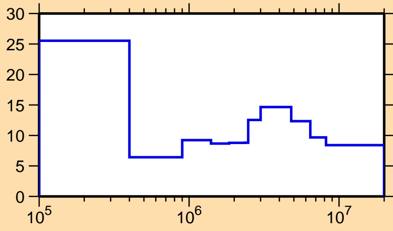
\Delta\sigma/\sigma vs. E for ^{151}\text{Dy}(n,\text{tot.})
