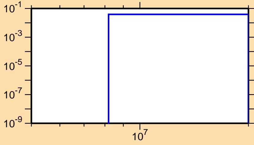
\sigma vs. E for ^{151}\text{Dy}(n,2n\alpha)
