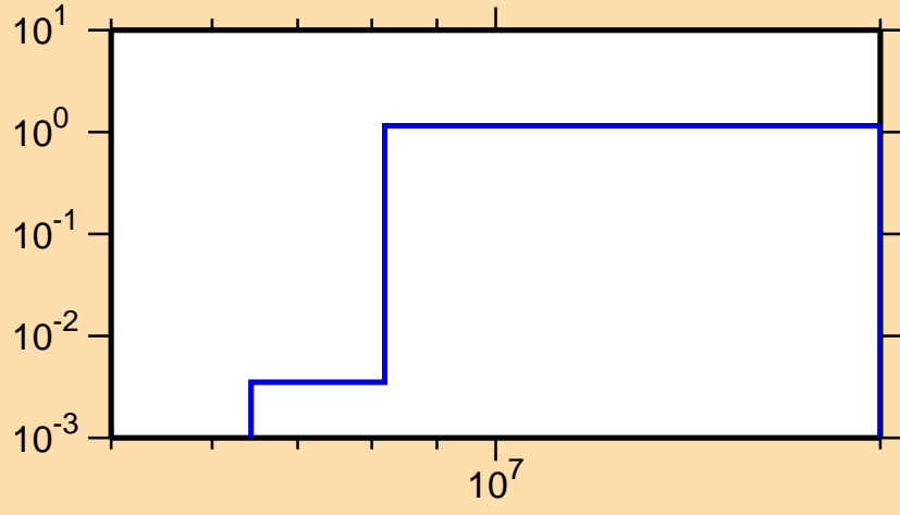
\sigma vs. E for ^{151}\text{Dy}(n,2n)
