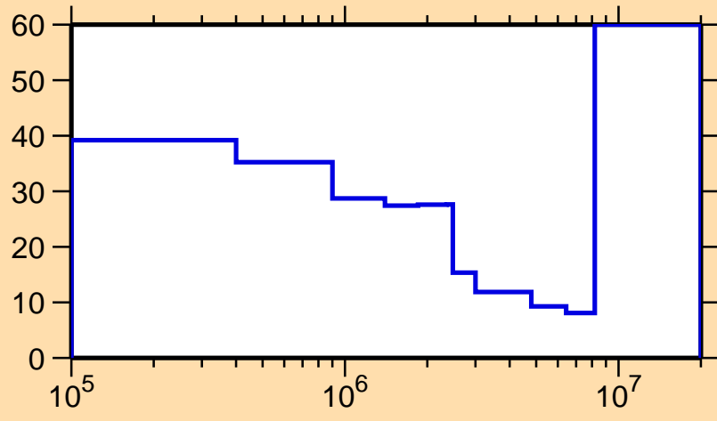
\Delta\sigma/\sigma vs. E for ^{151}\text{Dy}(n,\text{inel.})
