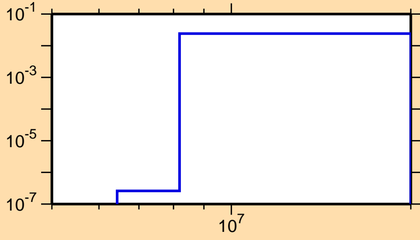
\sigma vs. E for ^{151}\text{Dy}(n,np)
