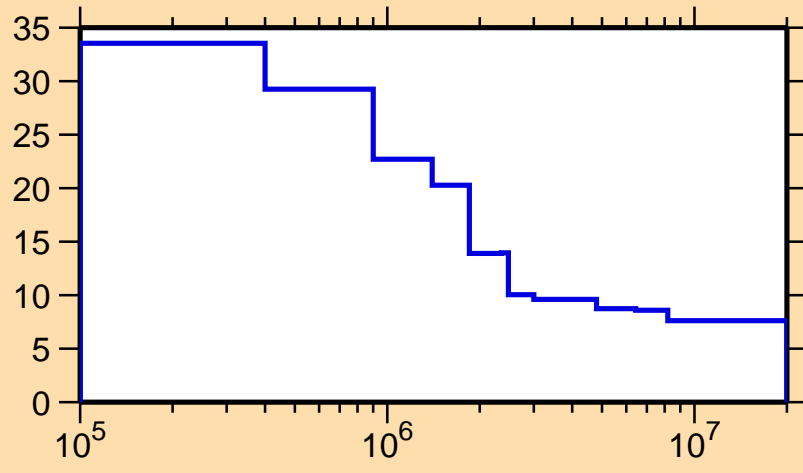
\Delta\sigma/\sigma vs. E for ^{151}\text{Dy}(n,\text{nonel.})
