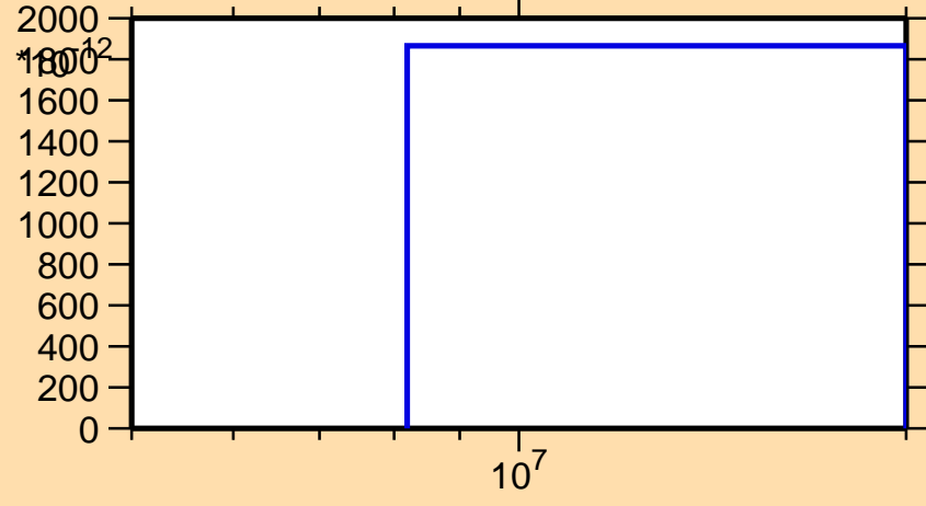
\sigma vs. E for ^{151}\text{Dy}(n,pd)
