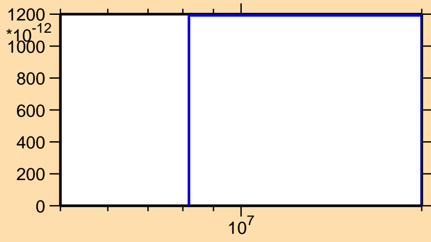
\sigma vs. E for ^{151}\text{Dy}(n,\text{pt})
