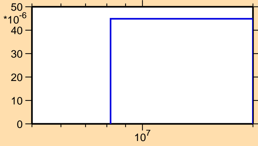
\sigma vs. E for ^{151}\text{Dy}(n,3n)
