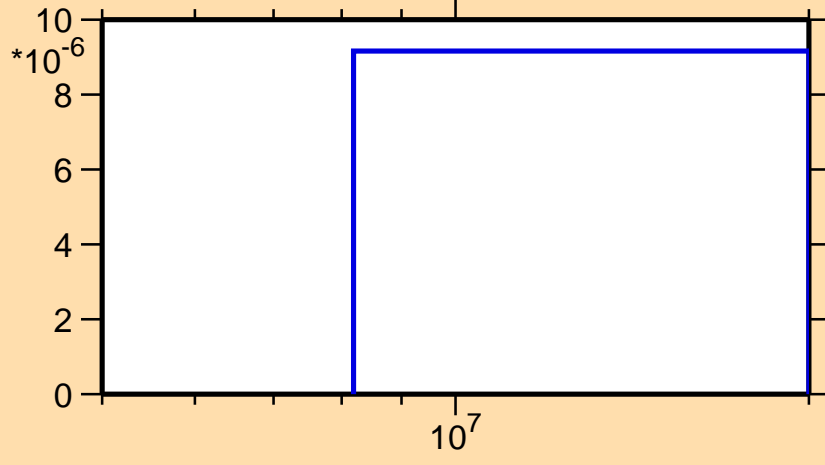
\sigma vs. E for ^{151}\text{Dy}(n,2np)
