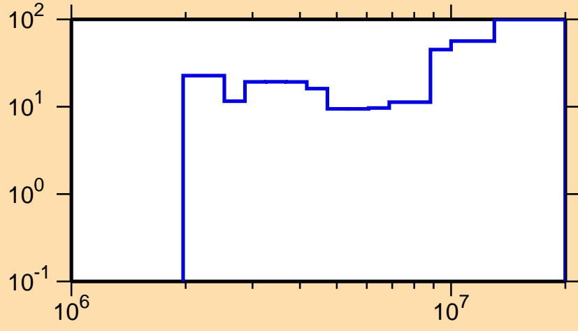
\Delta\sigma/\sigma vs. E for ^{152}\text{Dy}(n,inel.)
